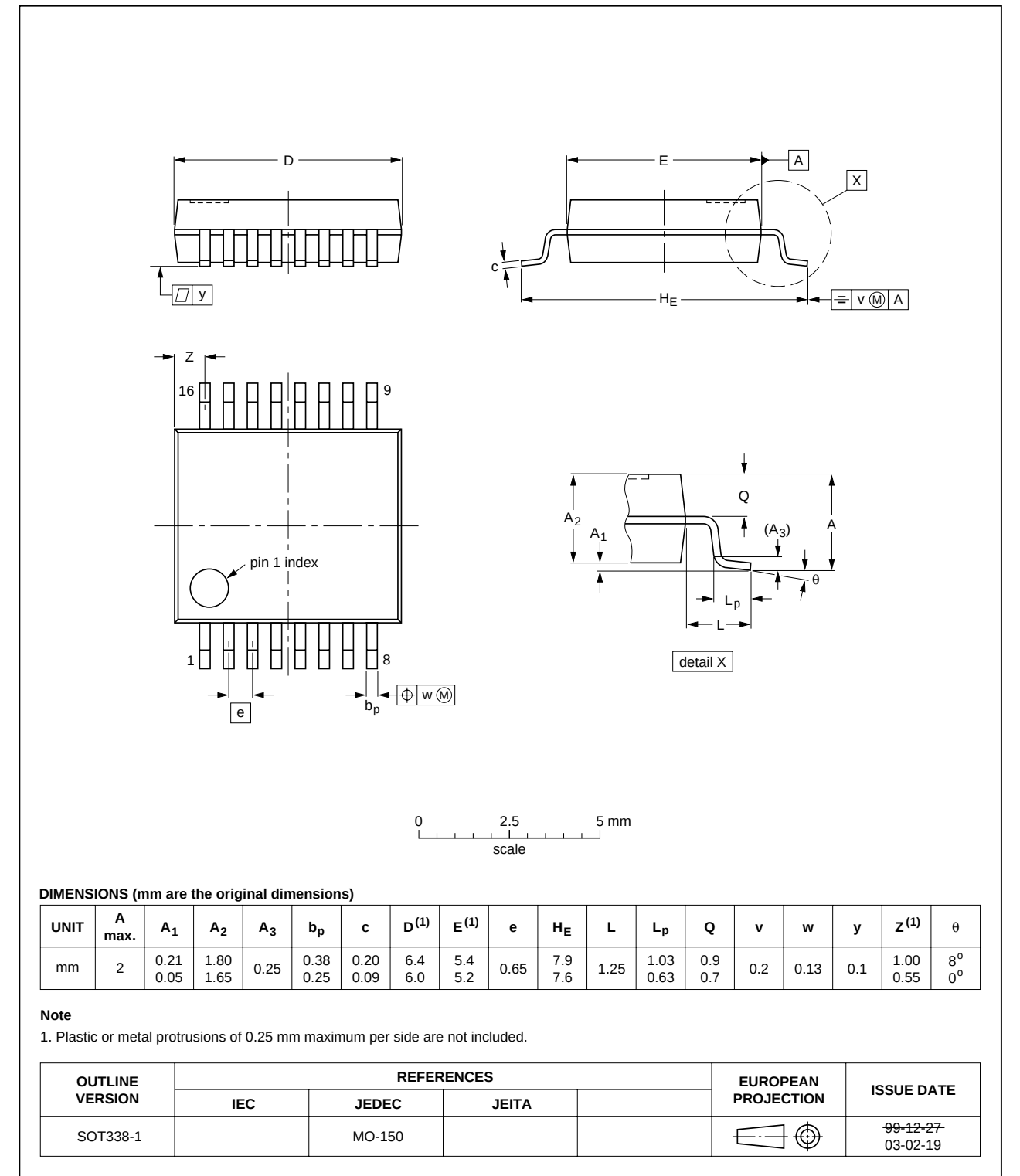
Fig 13. Package outline SOT338-1 (SSOP16)
